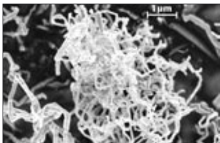
Carbon nanofilaments , produced during the solar thermal decomposition of methane. One example of the use of these nanofilaments is for composite materials. (Scanning electron micrograph, 1 μm = 1 micrometer = 1 thousandth of a millimetre)
