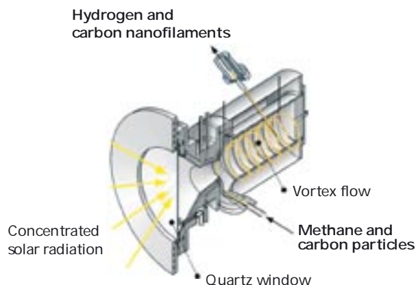
The solar chemical reactor features a vortex flow of methane confined to a cavity-receiver and laden with carbon particles. The source of high-temperature energy is concentrated sunlight. The chemical products are hydrogen and carbon nanofilaments. A schematic view is shown above, while the picture on the left shows the reactor installed in the PSI solar furnace.
